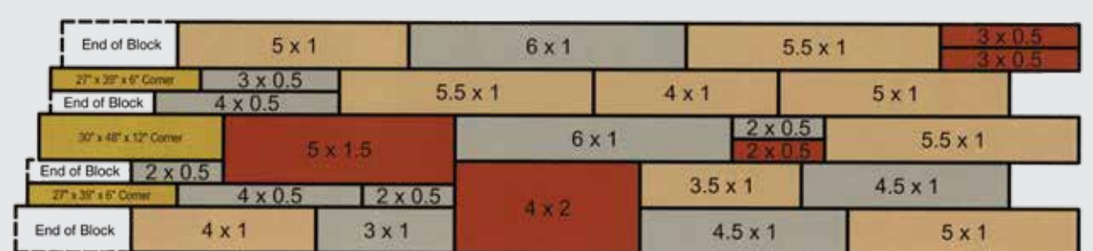
90° WALL CORNER
